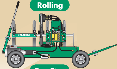
In-Ditch Fusion All Machines
