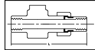
Insulated Union
