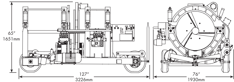
weight 4,500lbs (2041Kg) input power 30 KVA
