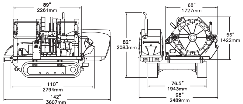
weight 9,300lbs (4218Kg) diesel - Self-Contained
